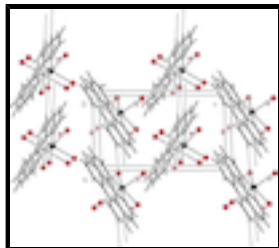
Fig. 2. View of the unit-cell contents of the title complex. Intermolecular hydrogen-bond interactions are drawn with dashed lines.
